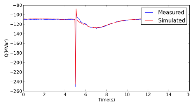
Figure 5 Example of reactive power comparison
