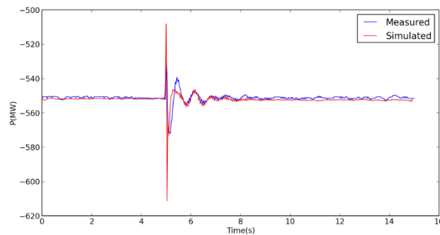
Figure 4 Example of real power comparison
